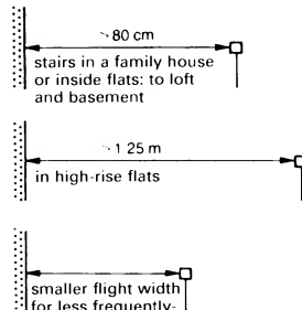
⑮ Measuring the effective flight width
